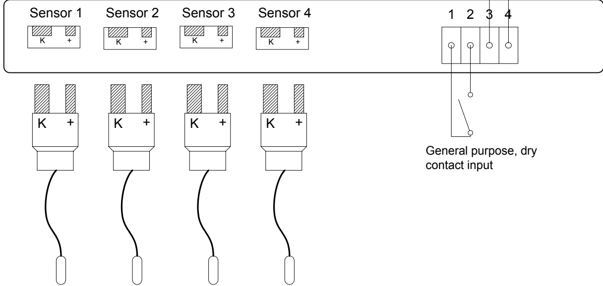
K type thermocouples with integrated spade connectors
